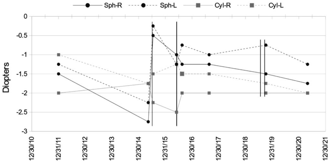
FIG. 6. Eyesight correction—Subject is nearsighted. Spherical (Sph) correction is the nearsighted or farsighted correction for the whole lens of the eye. A correction of zero is 20/20 vision. Cylindrical (Cyl) correction is for astigmatism and has an angle. Astigmatism angle differences (not shown) were within the range of measurement error.
